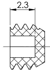
SECTION X-X
