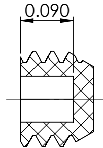
SECTION X-X
